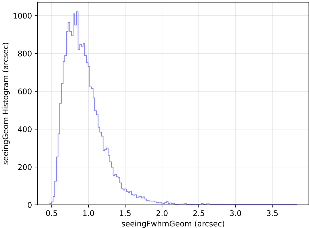
extra_ss_neo4_v3.4_10yrs Yr 1 g band: seeingGeom Histogram
