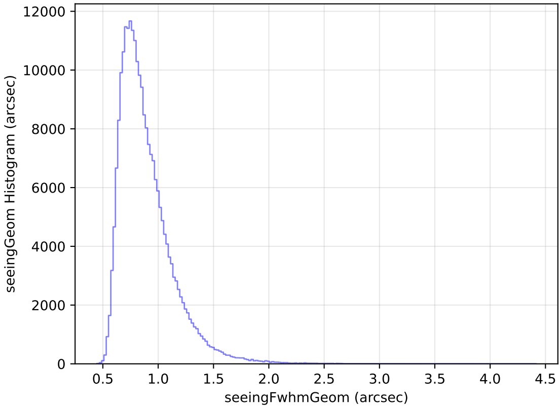
extra_ss_neo4_v3.4_10yrs Yr 1 all bands: seeingGeom Histogram
