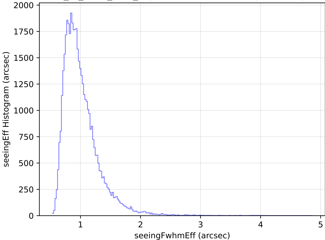
extra_ss_neo4_v3.4_10yrs Yr 1 z band: seeingEff Histogram
