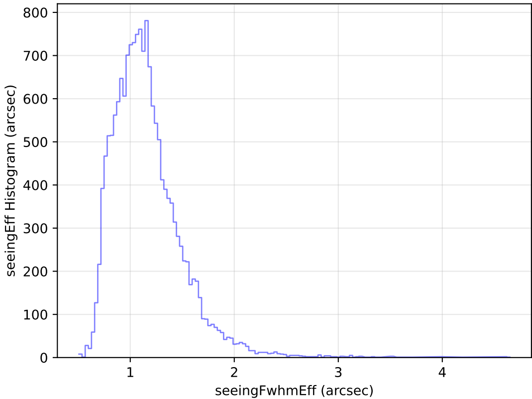
extra_ss_neo4_v3.4_10yrs Yr 1 u band: seeingEff Histogram
