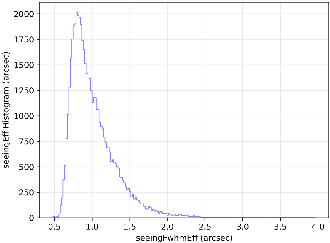
extra_ss_neo4_v3.4_10yrs Yr 1 r band: seeingEff Histogram
