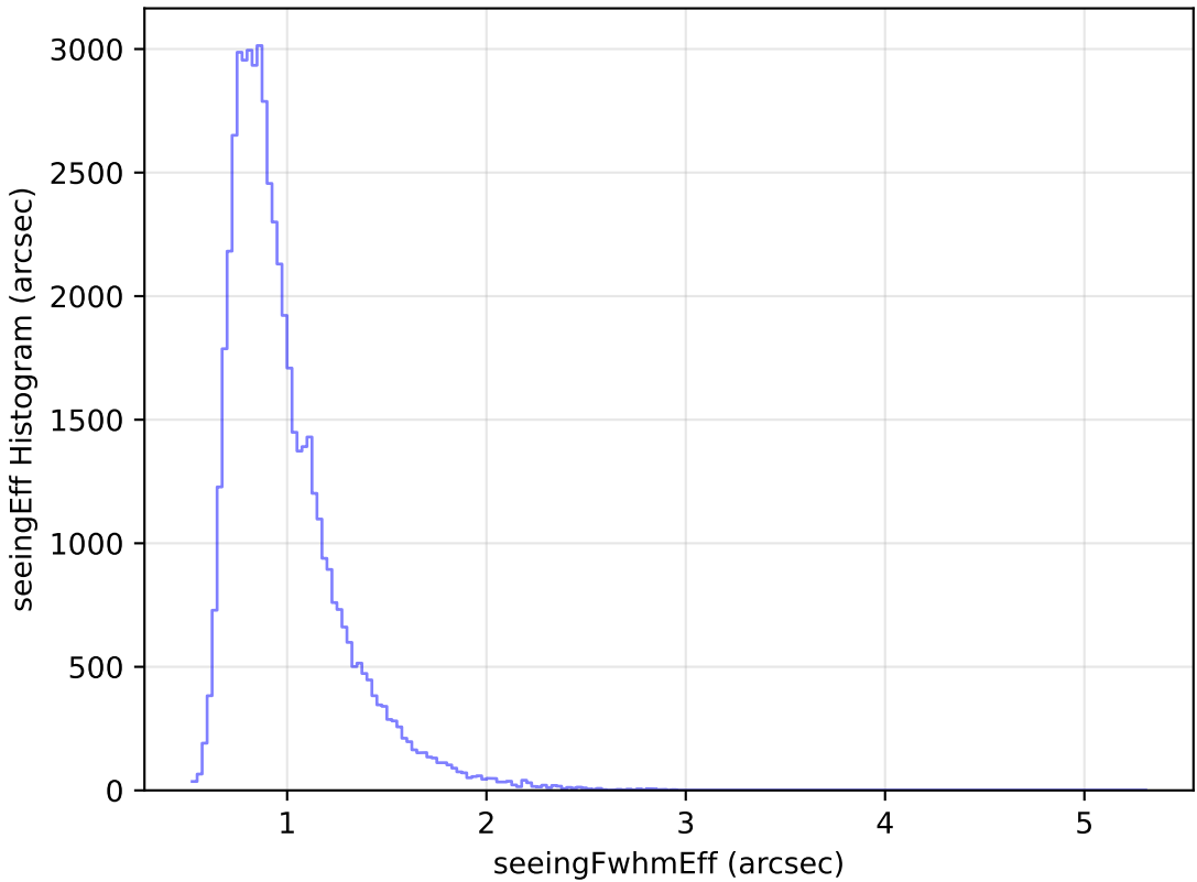
extra_ss_neo4_v3.4_10yrs Yr 1 i band: seeingEff Histogram
