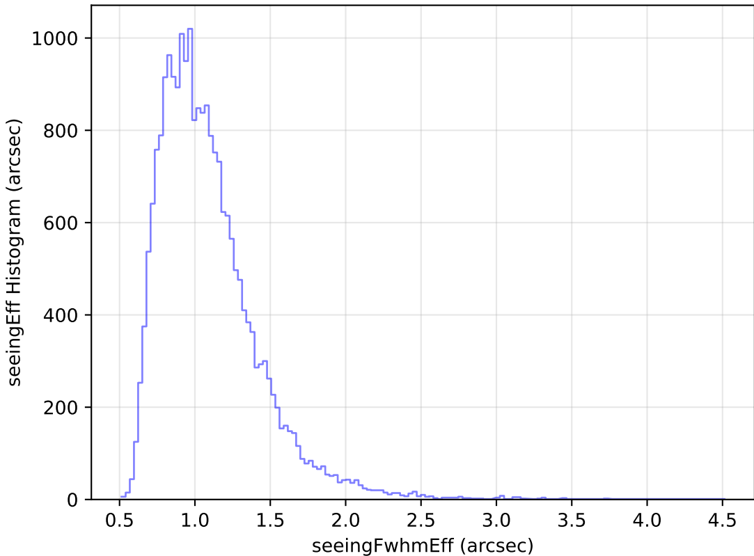
extra_ss_neo4_v3.4_10yrs Yr 1 g band: seeingEff Histogram
