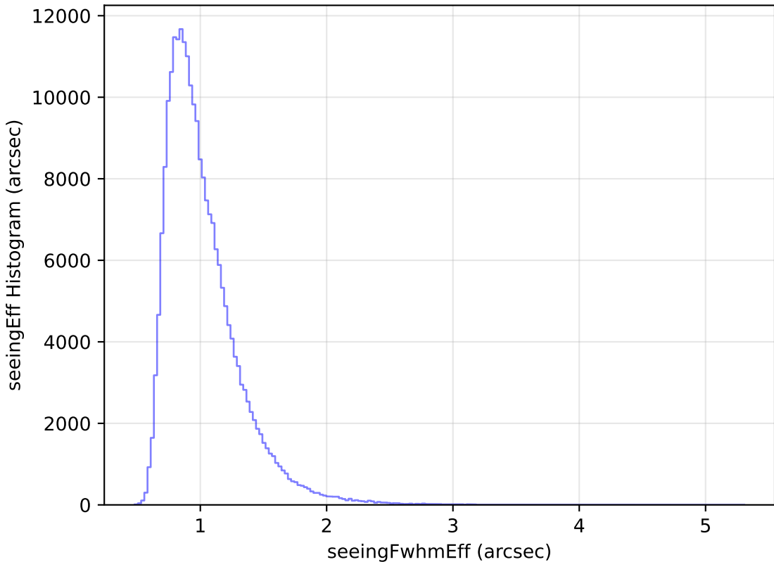
extra_ss_neo4_v3.4_10yrs Yr 1 all bands: seeingEff Histogram
