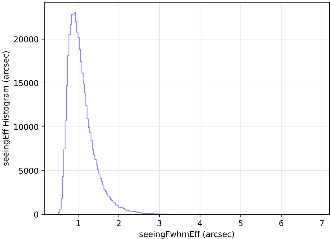
extra_ss_neo4_v3.4_10yrs WFD z band: seeingEff Histogram
