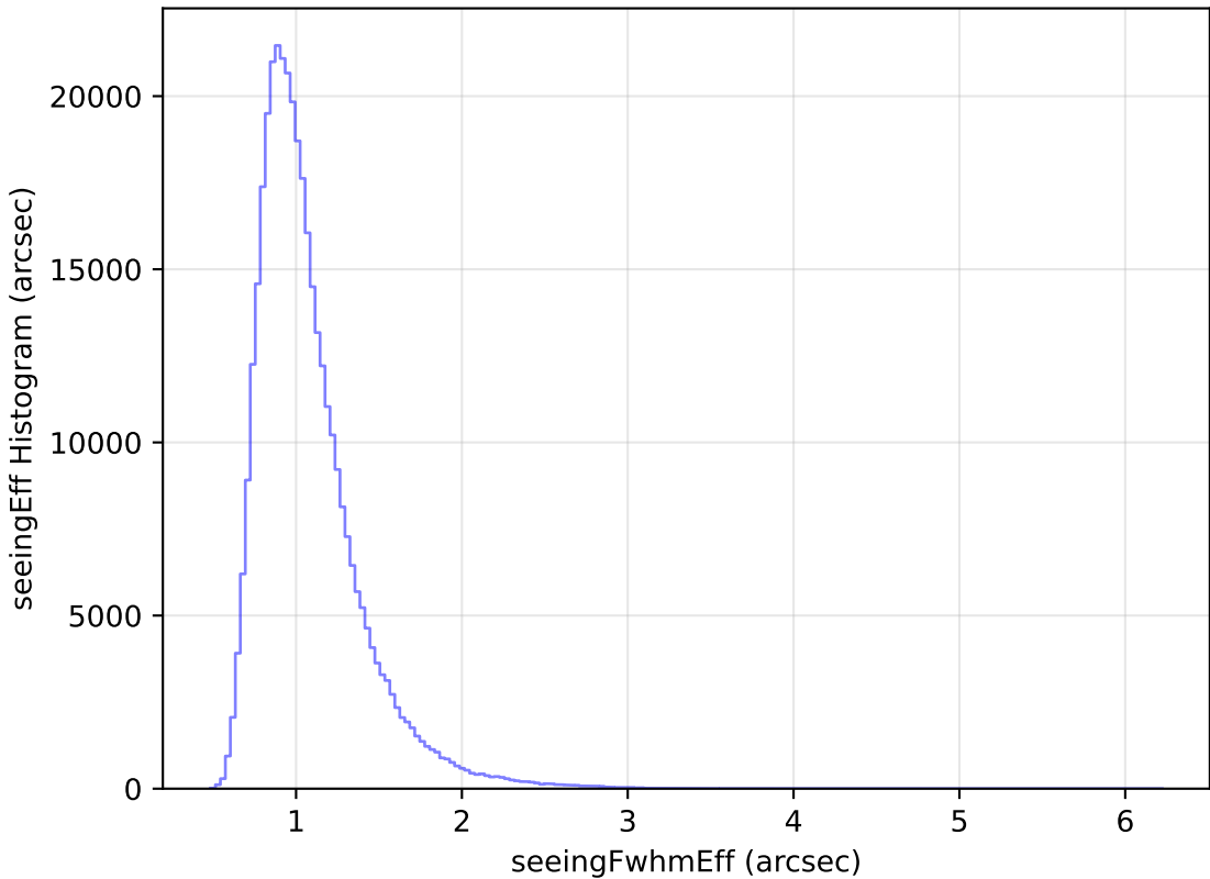
extra_ss_neo4_v3.4_10yrs WFD y band: seeingEff Histogram
