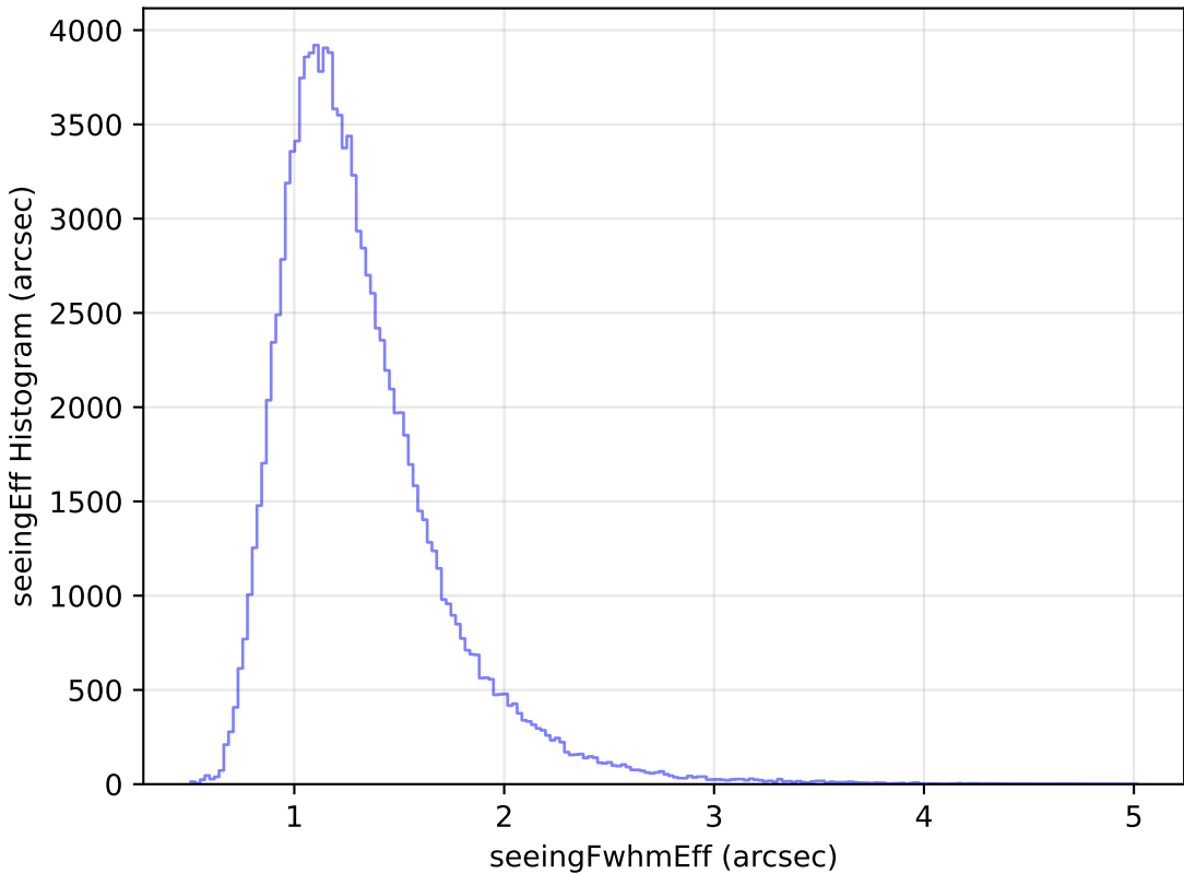
extra_ss_neo4_v3.4_10yrs WFD u band: seeingEff Histogram
