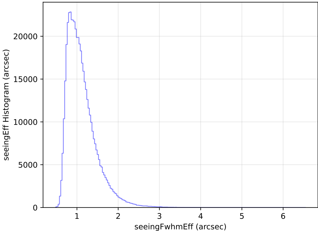
extra_ss_neo4_v3.4_10yrs WFD r band: seeingEff Histogram
