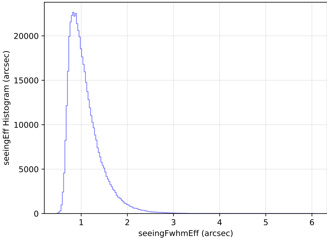
extra_ss_neo4_v3.4_10yrs WFD i band: seeingEff Histogram
