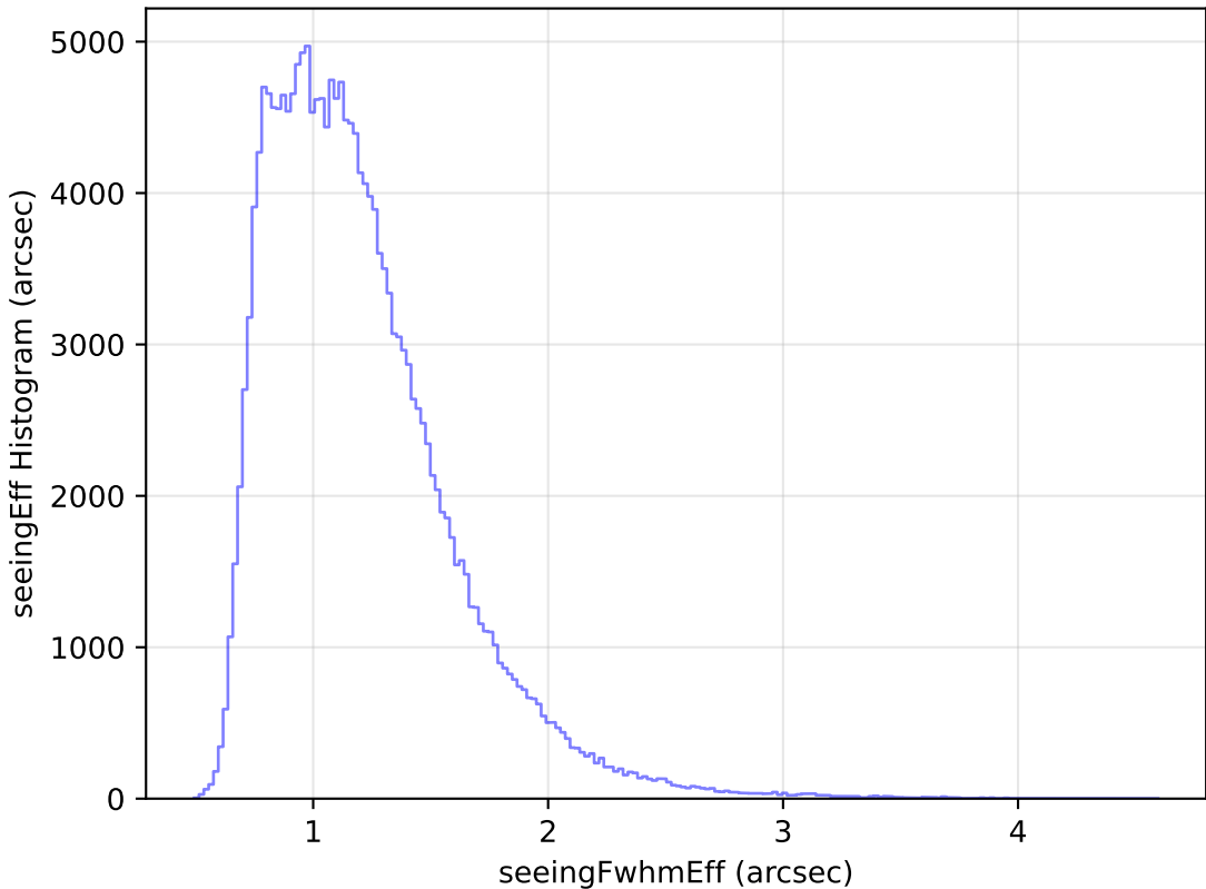
extra_ss_neo4_v3.4_10yrs WFD g band: seeingEff Histogram
