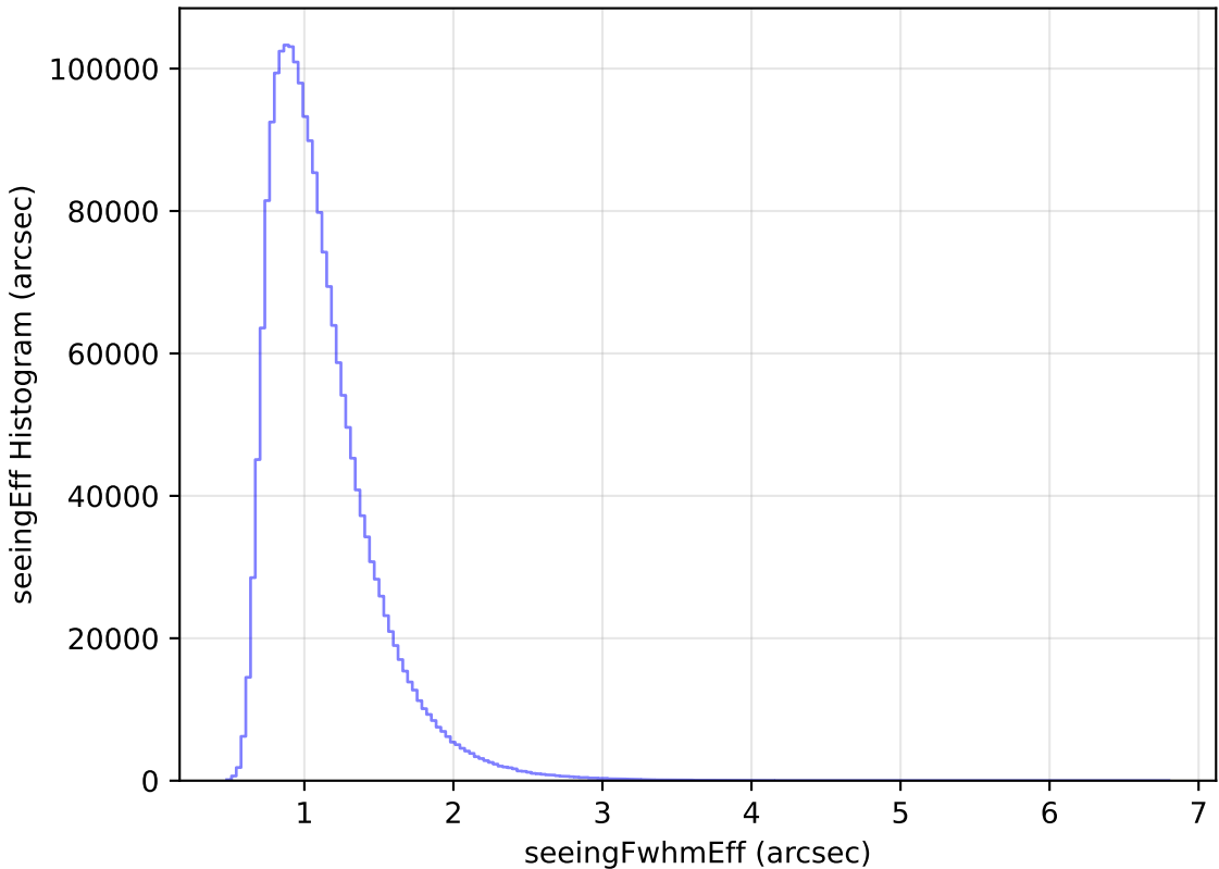
extra_ss_neo4_v3.4_10yrs WFD all bands: seeingEff Histogram
