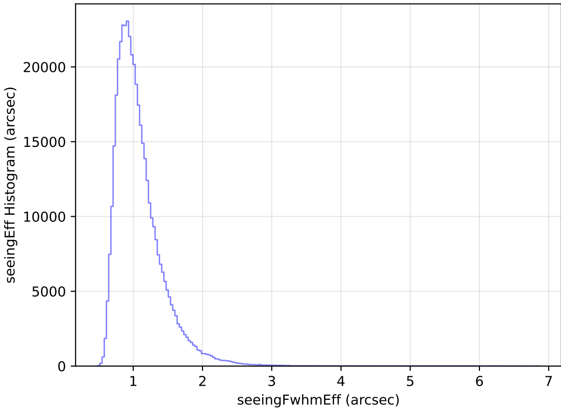
extra_ss_neo4_v3.4_10yrs All sky z band: seeingEff Histogram
