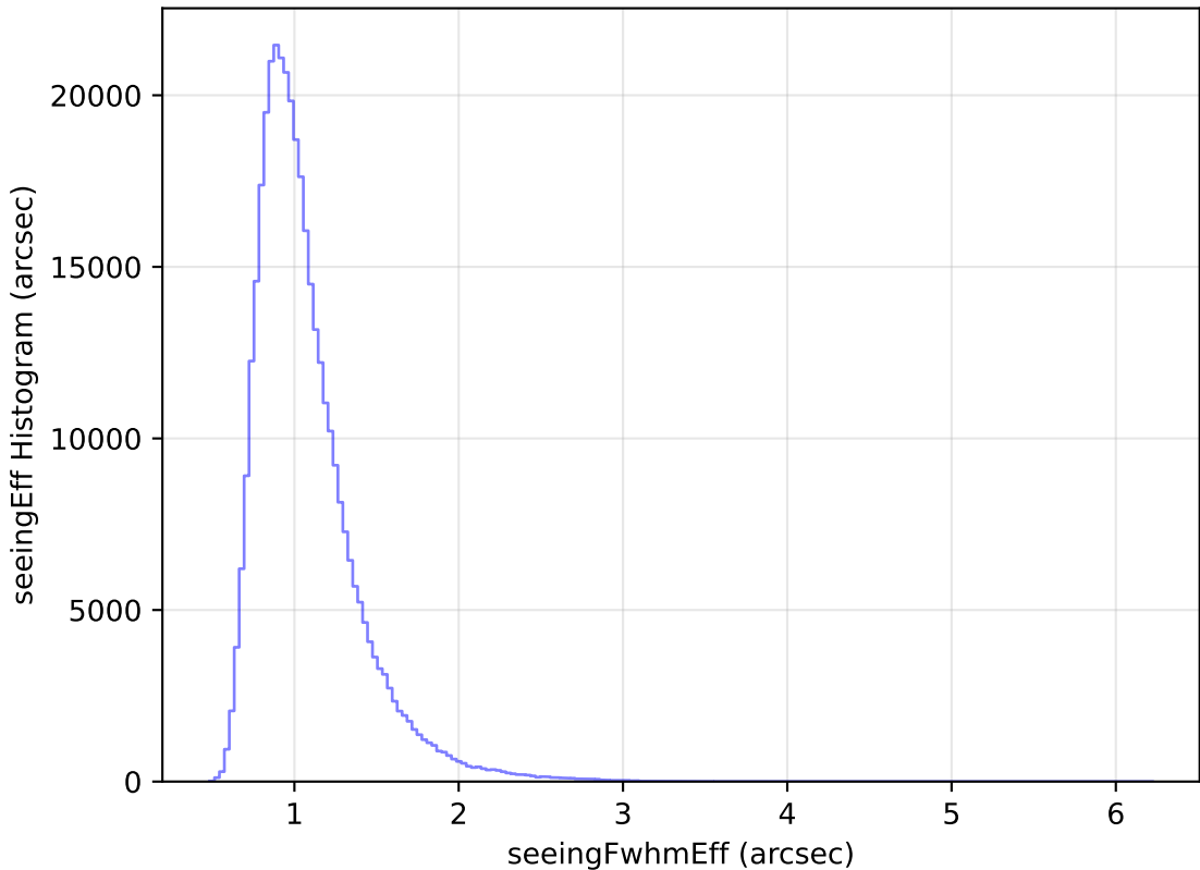
extra_ss_neo4_v3.4_10yrs All sky y band: seeingEff Histogram
