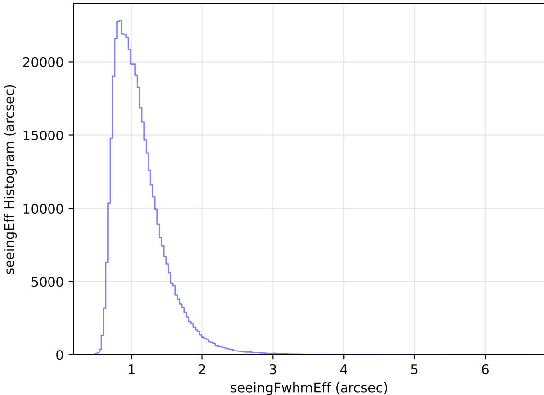
extra_ss_neo4_v3.4_10yrs All sky r band: seeingEff Histogram
