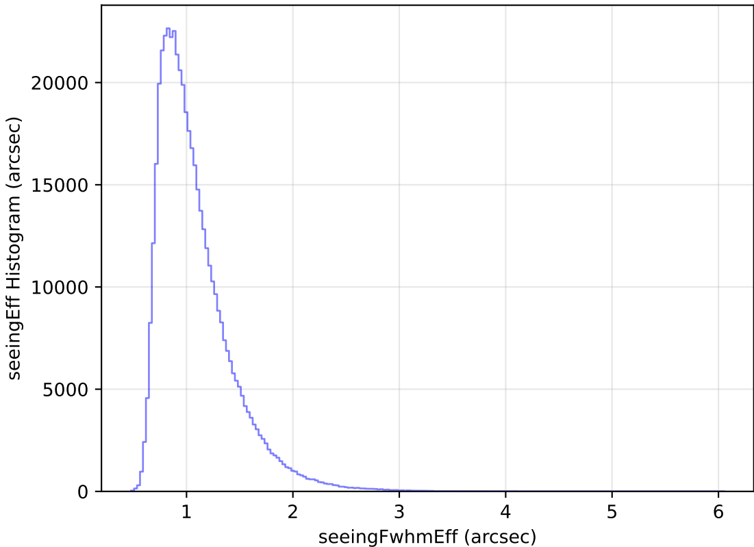
extra_ss_neo4_v3.4_10yrs All sky i band: seeingEff Histogram
