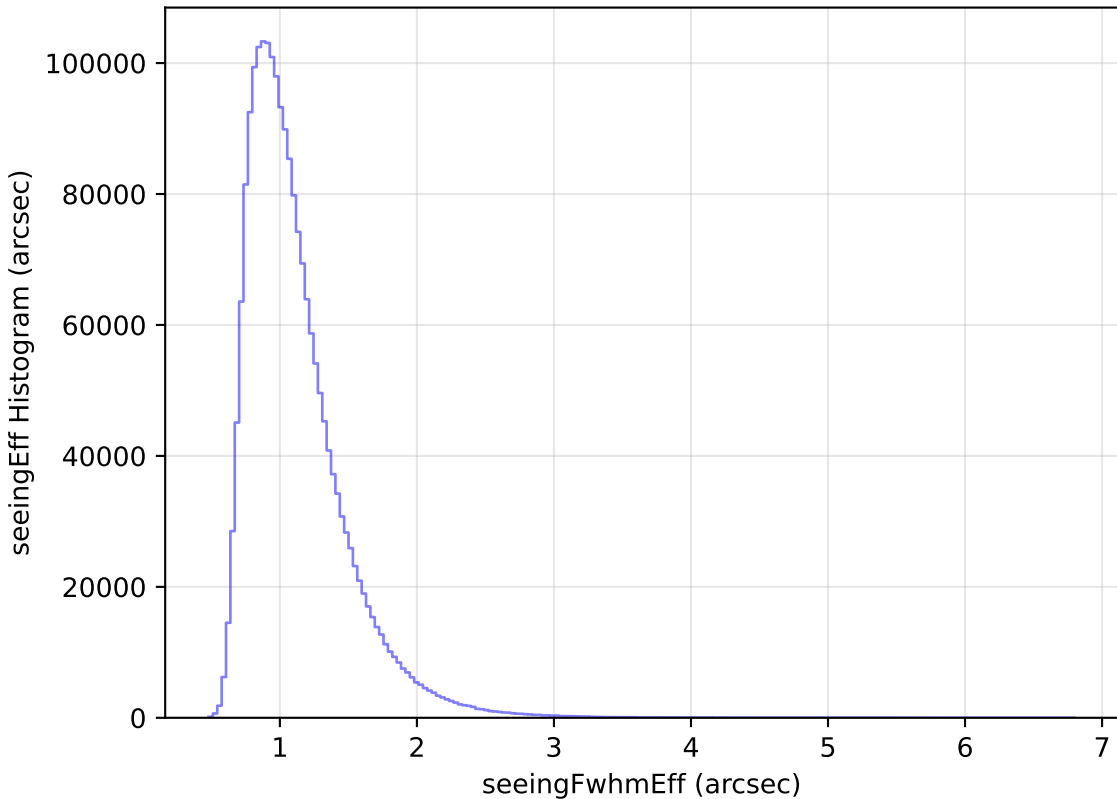
extra_ss_neo4_v3.4_10yrs All sky all bands: seeingEff Histogram
