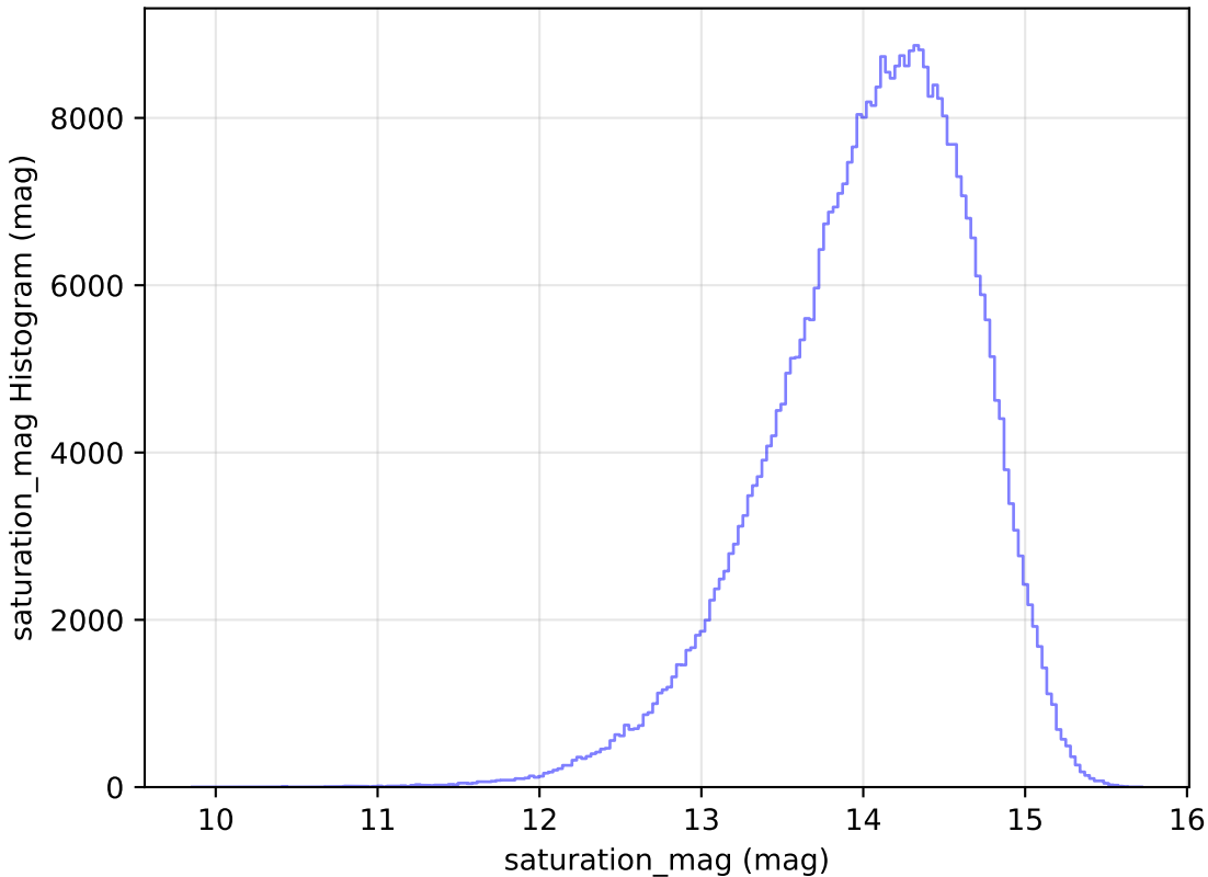
extra_ss_neo4_v3.4_10yrs WFD z band: saturation_mag Histogram
