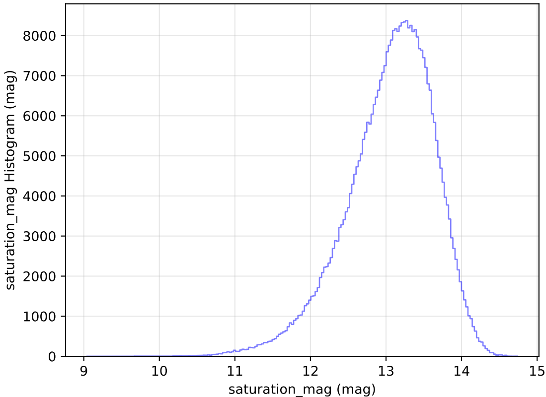
extra_ss_neo4_v3.4_10yrs WFD y band: saturation_mag Histogram
