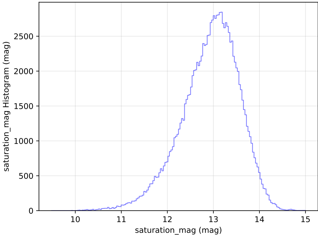
extra_ss_neo4_v3.4_10yrs WFD u band: saturation_mag Histogram
