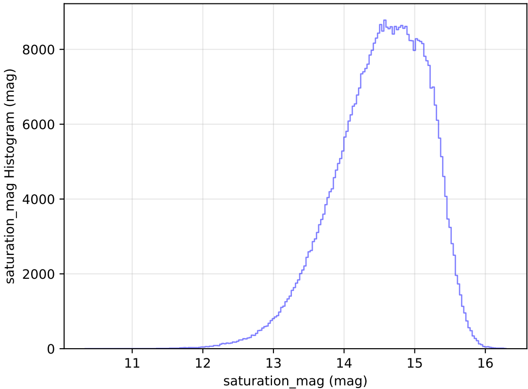
extra_ss_neo4_v3.4_10yrs WFD r band: saturation_mag Histogram
