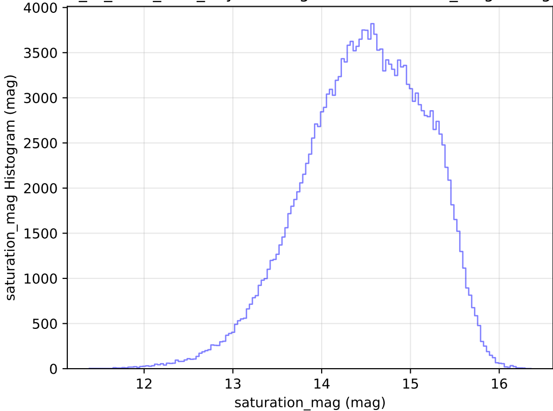
extra_ss_neo4_v3.4_10yrs WFD g band: saturation_mag Histogram
