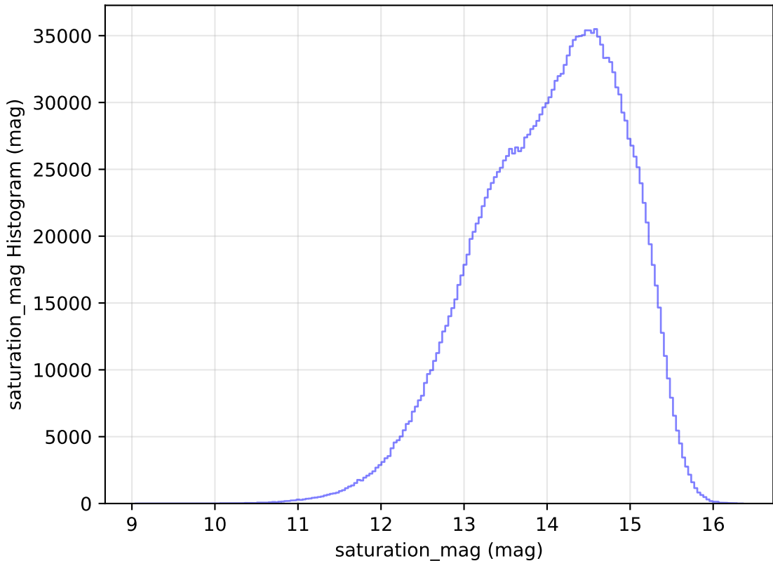
extra_ss_neo4_v3.4_10yrs WFD all bands: saturation_mag Histogram
