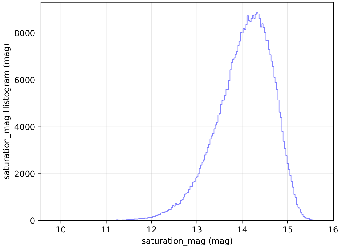
extra_ss_neo4_v3.4_10yrs All sky z band: saturation_mag Histogram
