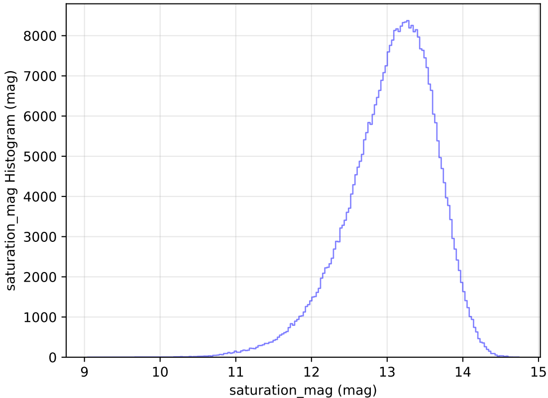
extra_ss_neo4_v3.4_10yrs All sky y band: saturation_mag Histogram
