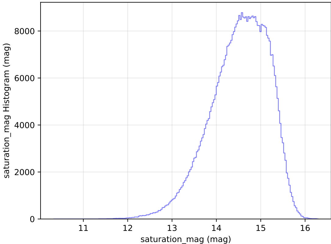
extra_ss_neo4_v3.4_10yrs All sky r band: saturation_mag Histogram
