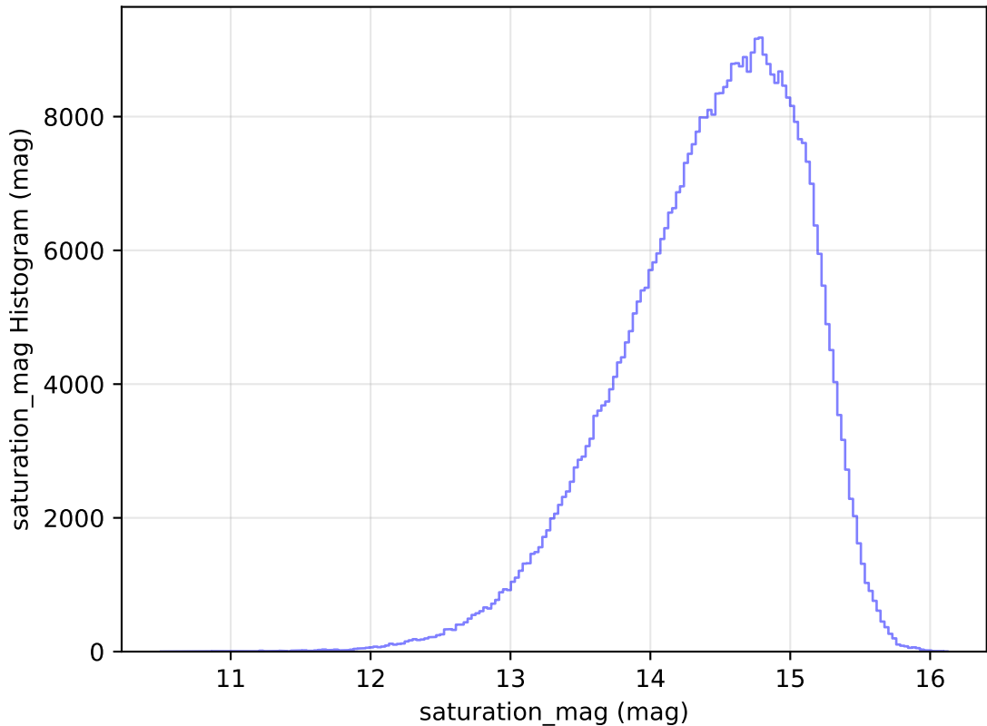
extra_ss_neo4_v3.4_10yrs All sky i band: saturation_mag Histogram
