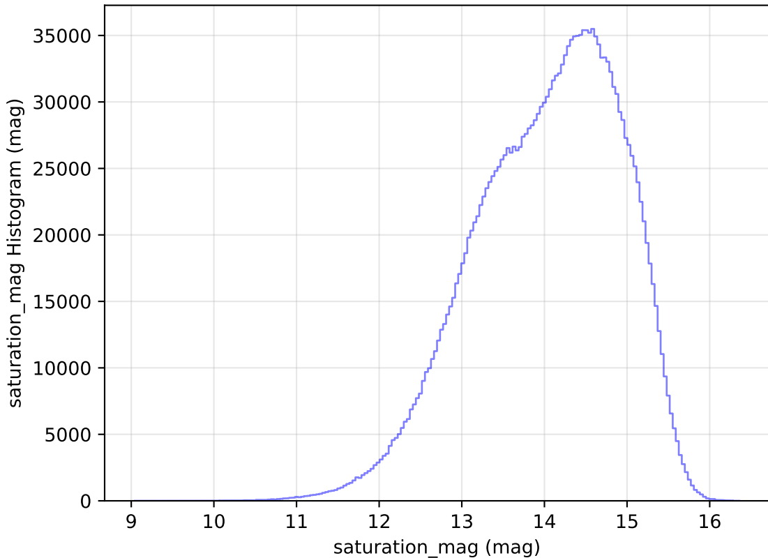
extra_ss_neo4_v3.4_10yrs All sky all bands: saturation_mag Histogram
