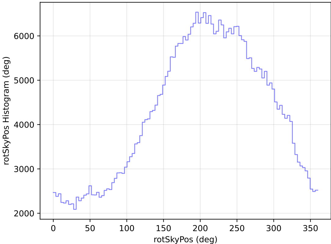
extra_ss_neo4_v3.4_10yrs WFD z band: rotSkyPos Histogram
