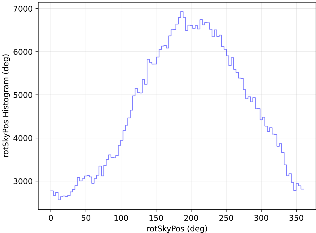
extra_ss_neo4_v3.4_10yrs WFD r band: rotSkyPos Histogram
