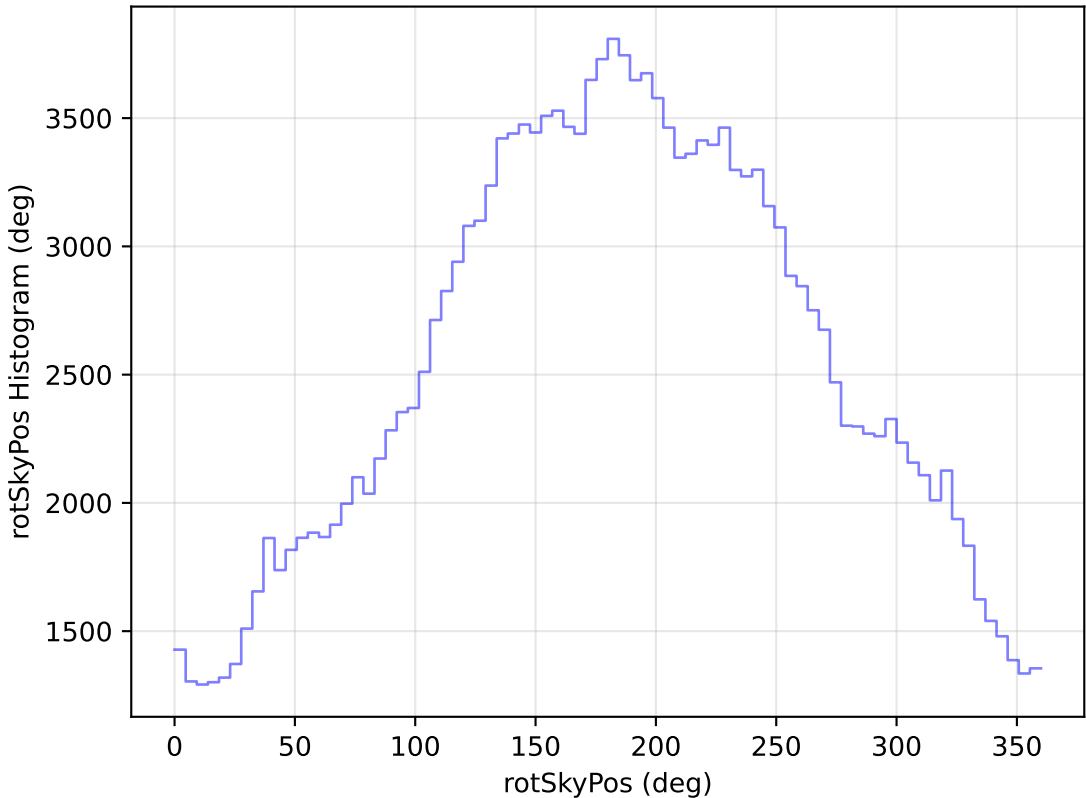
extra_ss_neo4_v3.4_10yrs WFD g band: rotSkyPos Histogram
