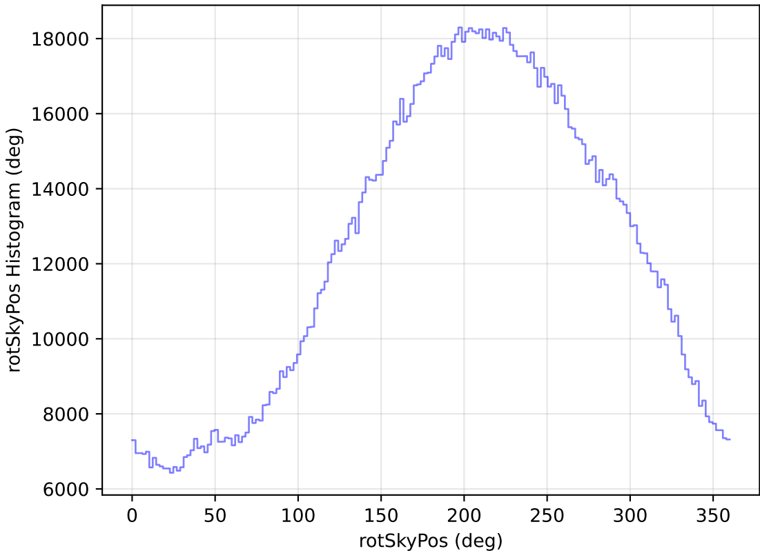
extra_ss_neo4_v3.4_10yrs WFD all bands: rotSkyPos Histogram
