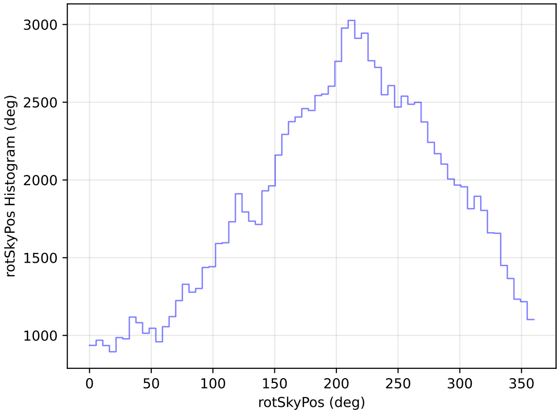
extra_ss_neo4_v3.4_10yrs All sky u band: rotSkyPos Histogram
