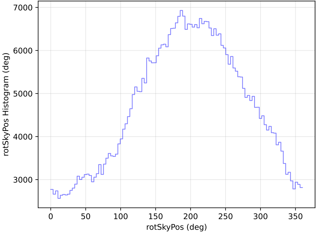
extra_ss_neo4_v3.4_10yrs All sky r band: rotSkyPos Histogram
