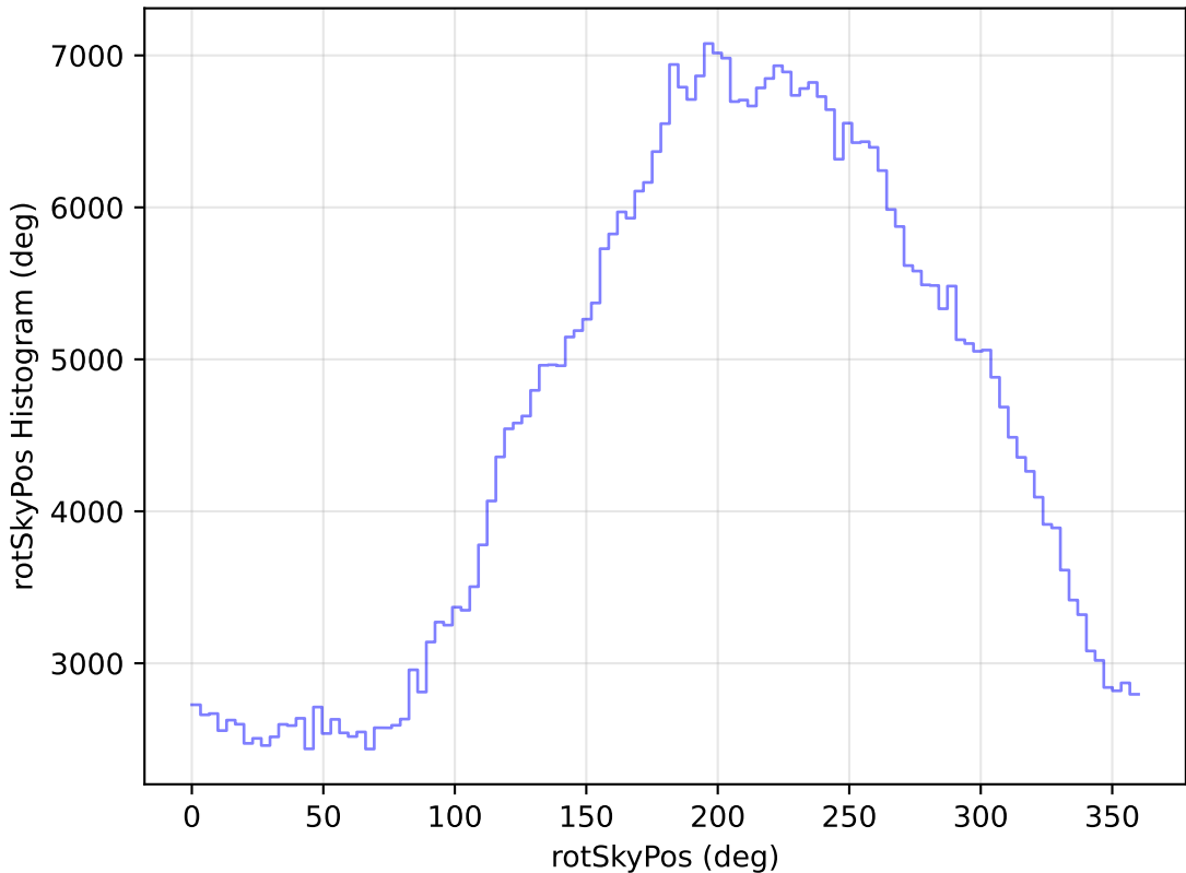
extra_ss_neo4_v3.4_10yrs All sky i band: rotSkyPos Histogram
