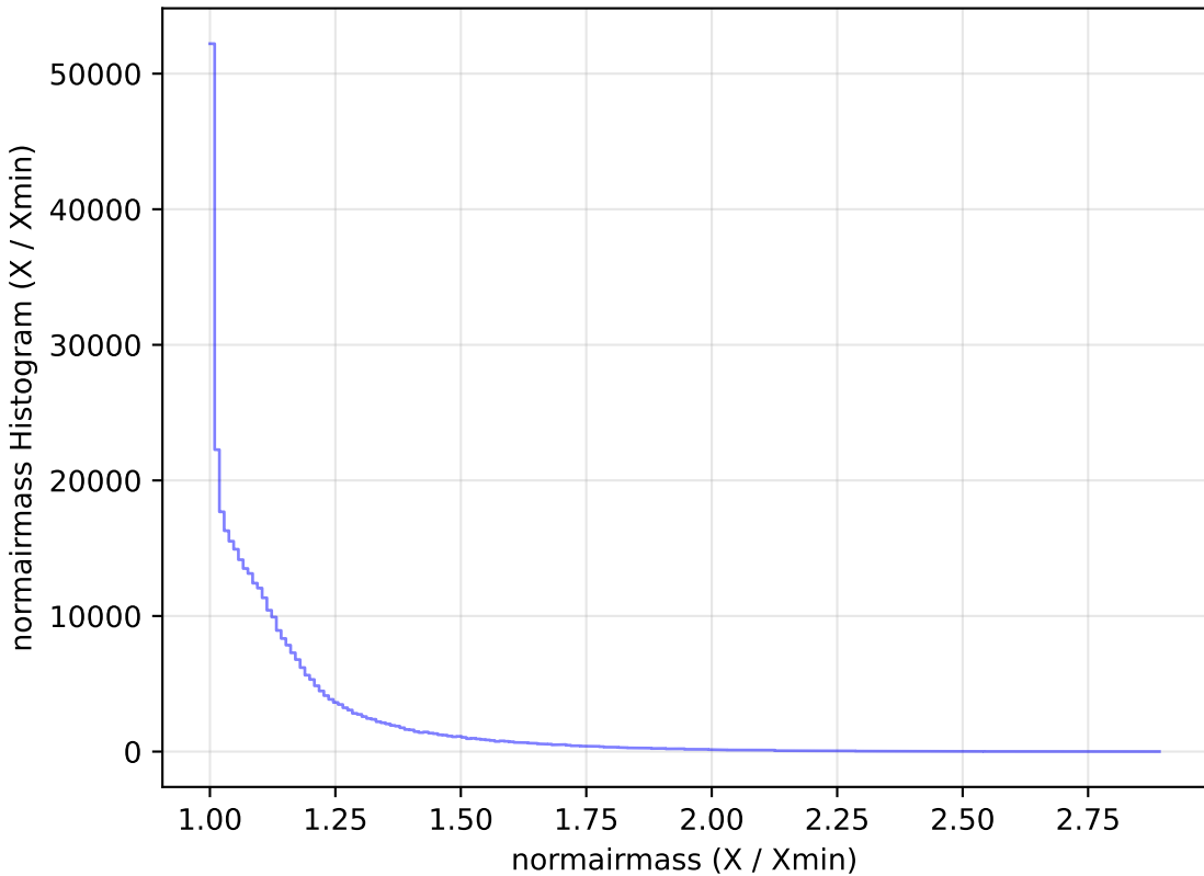
extra_ss_neo4_v3.4_10yrs WFD y band: normairmass Histogram
