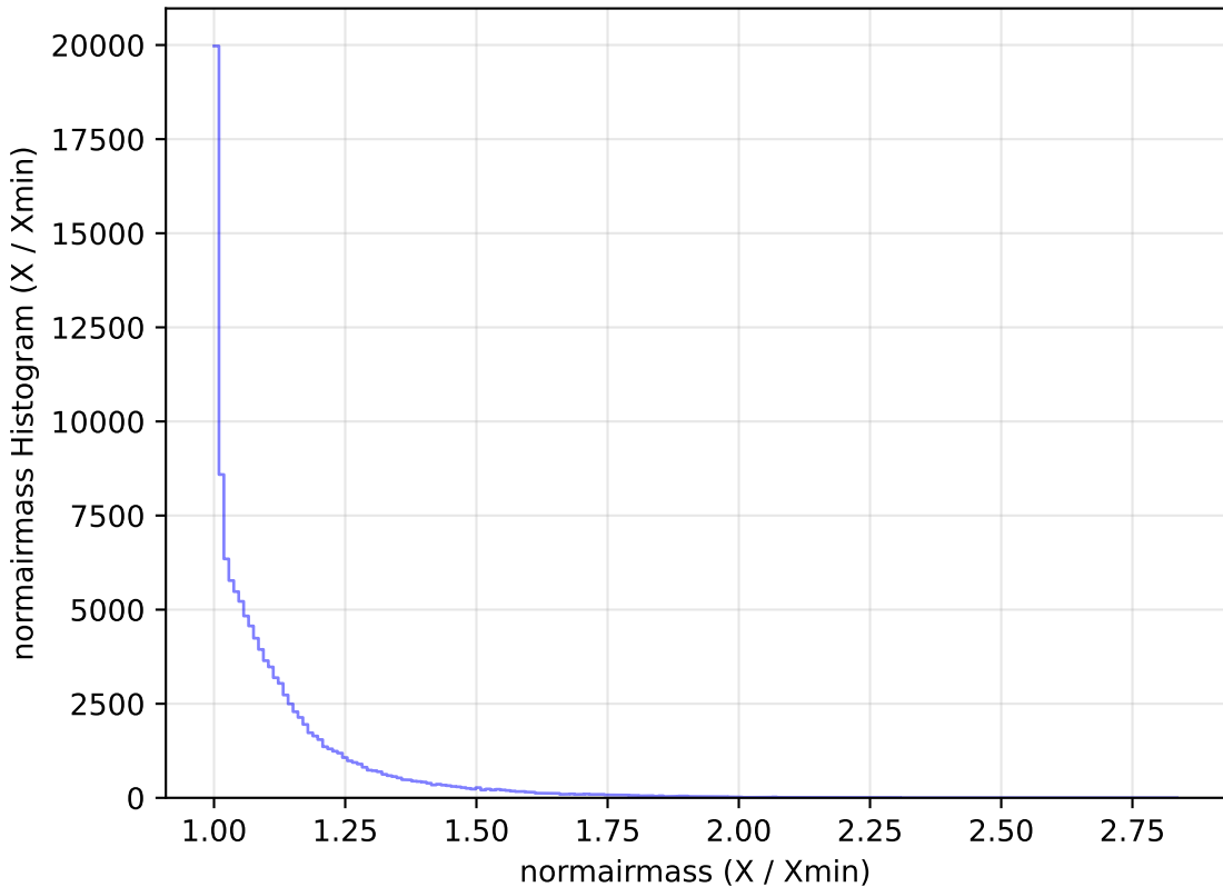
extra_ss_neo4_v3.4_10yrs WFD u band: normairmass Histogram
