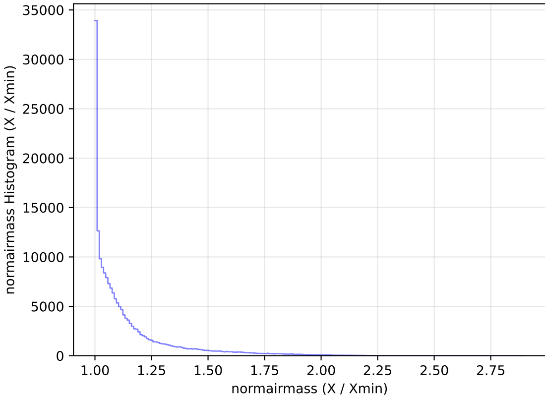
extra_ss_neo4_v3.4_10yrs WFD g band: normairmass Histogram
