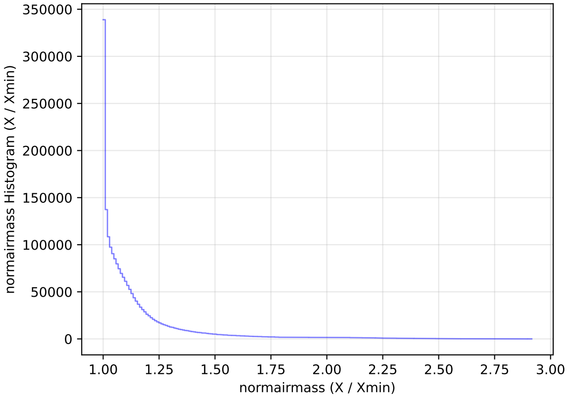
extra_ss_neo4_v3.4_10yrs WFD all bands: normairmass Histogram
