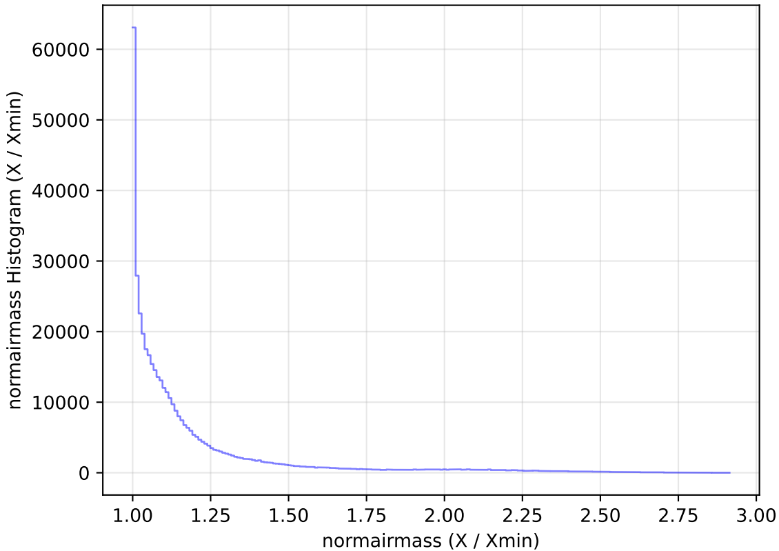
extra_ss_neo4_v3.4_10yrs All sky z band: normairmass Histogram
