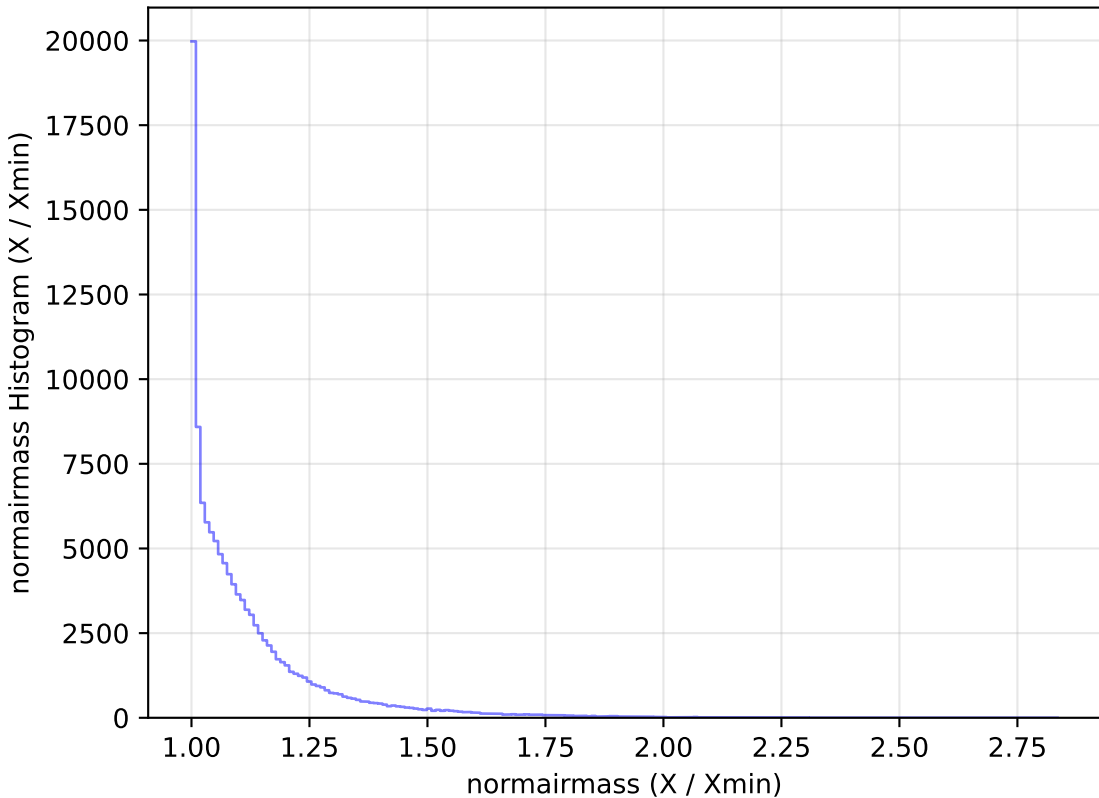
extra_ss_neo4_v3.4_10yrs All sky u band: normairmass Histogram
