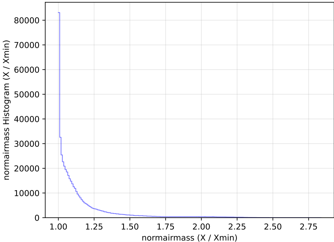
extra_ss_neo4_v3.4_10yrs All sky r band: normairmass Histogram
