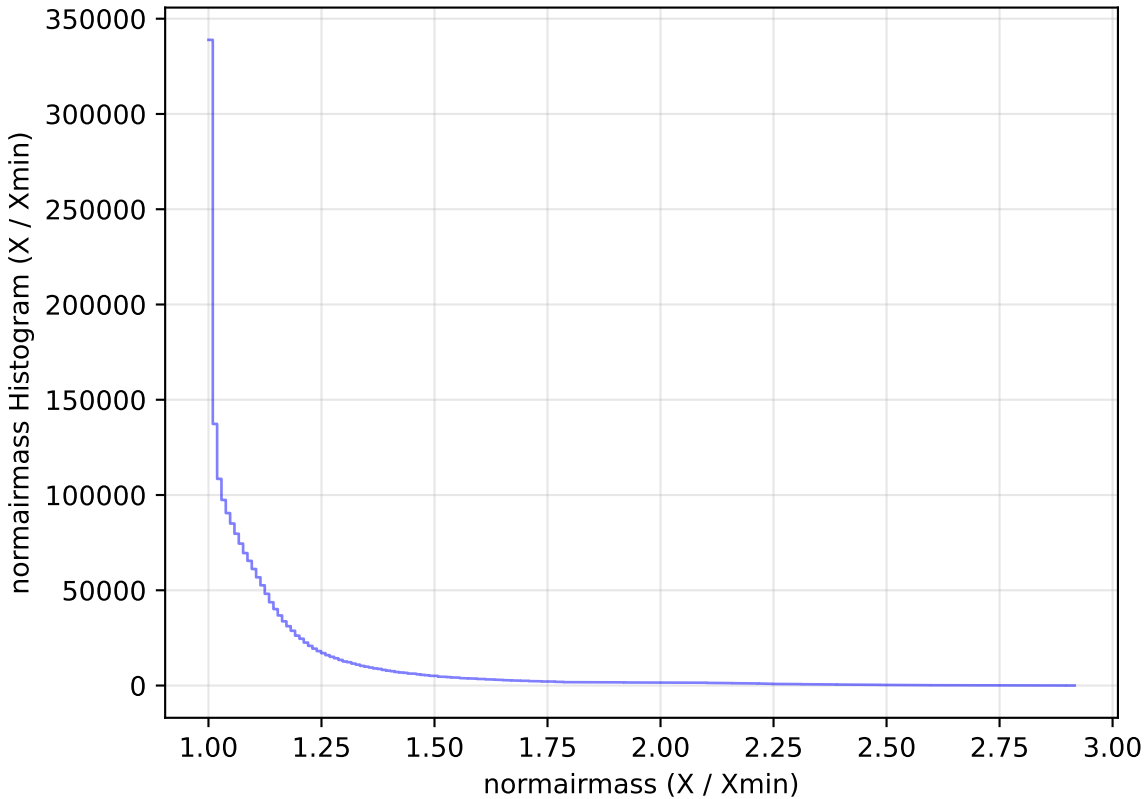
extra_ss_neo4_v3.4_10yrs All sky all bands: normairmass Histogram
