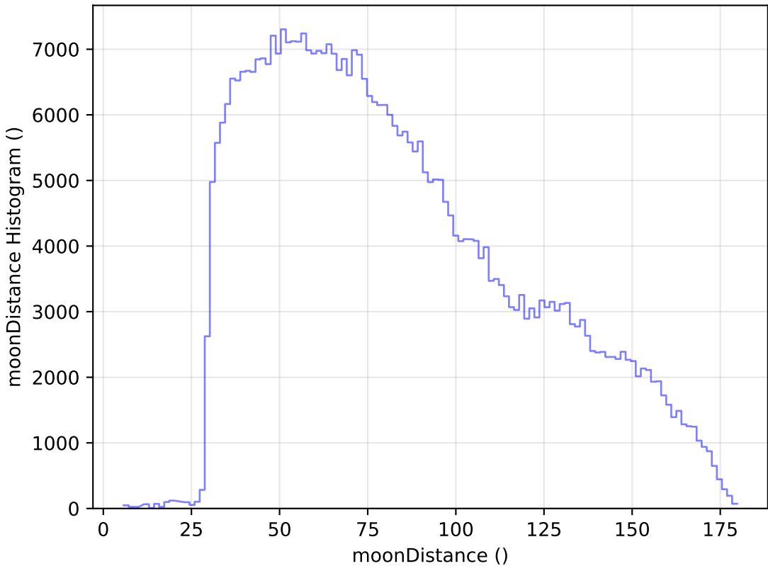
extra_ss_neo4_v3.4_10yrs WFD z band: moonDistance Histogram
