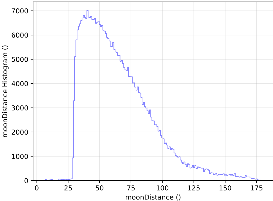
extra_ss_neo4_v3.4_10yrs WFD y band: moonDistance Histogram
