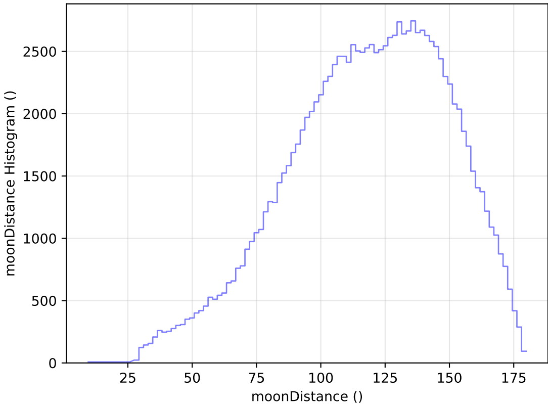
extra_ss_neo4_v3.4_10yrs WFD u band: moonDistance Histogram
