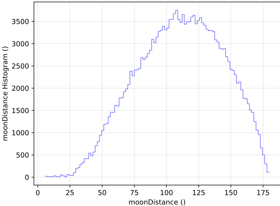
extra_ss_neo4_v3.4_10yrs WFD g band: moonDistance Histogram
